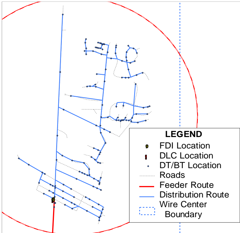
Figure 7—Distribution Plant
